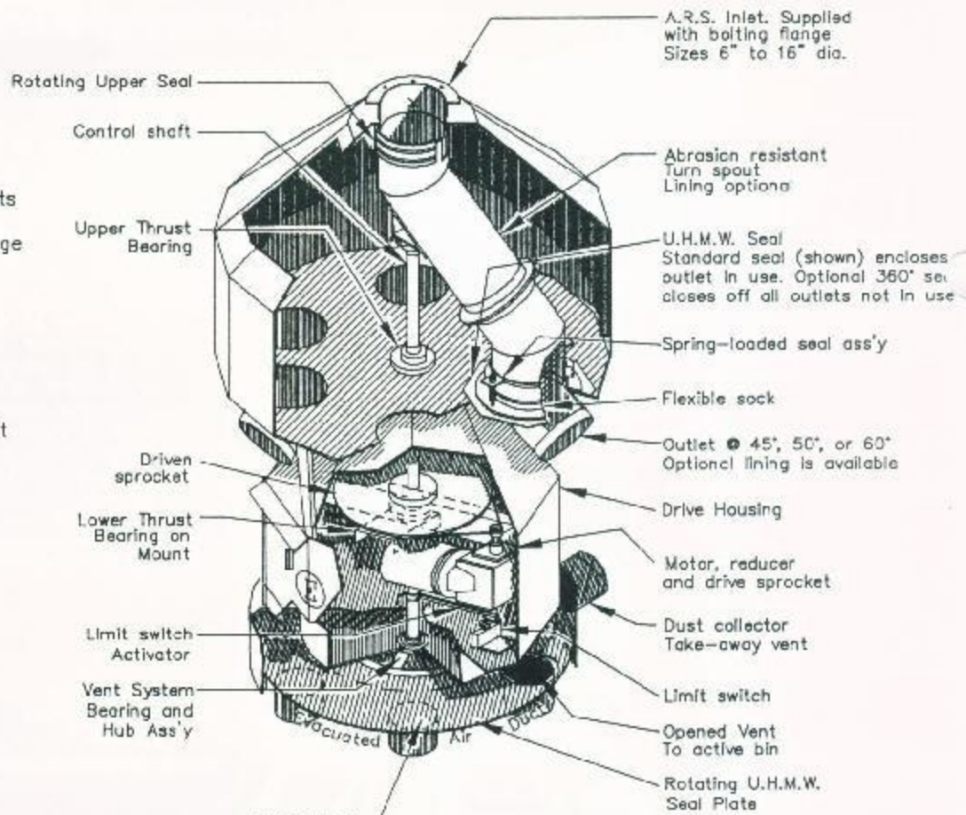
Cut-Away View of Turn-head Distributor With Directional Bin Vent System Option
