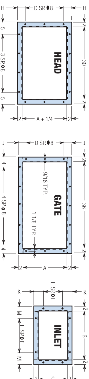
STANDARD FLANGE PATTERNS
