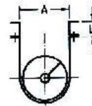
DIRECT INLET NON-FLARED INLET MAY BE OMITTED AND TROUGH BOLTED DIRECTLY TO HOPPER DISCHARGE FLANGE
